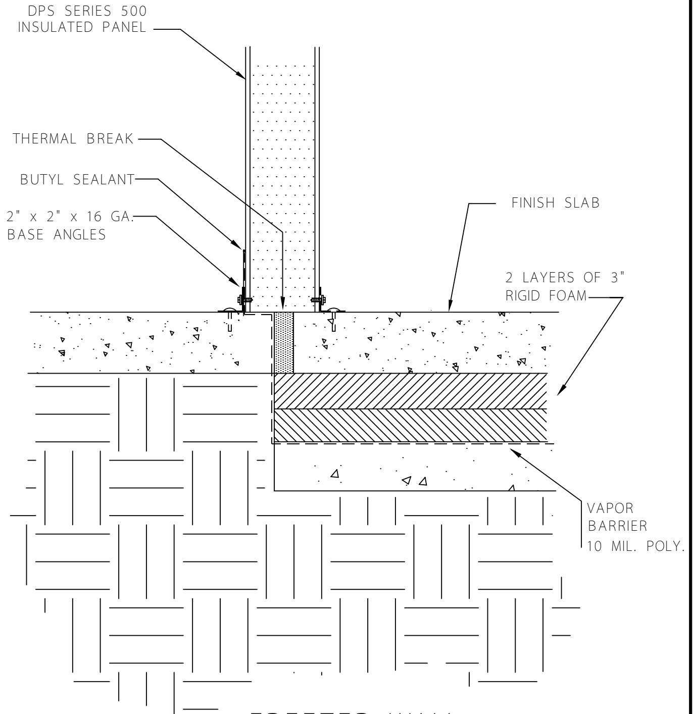
FREEZER WALL BASE DETAIL WITHOUT CURB
